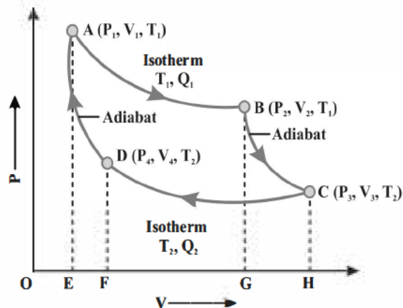
Figure 16.6 Carnot Cycle
