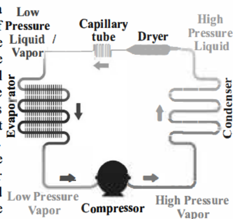
Figure 17.9 Refrigeration cycle
